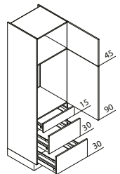
GKAK Appliance unit for refrigerator / recess 88 cm ↔ 60 ↓ 195/210/225 ↙ 60
