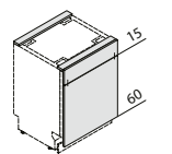
sSBS Front panel for fully integrated dishwashers
