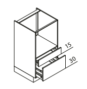
GBAS Appliance unit for oven or microwave ↳ 60 ↓ 105 ↶ 60
