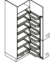
VVK Larder unit ↔ 60 ↓ 195/210/225 ↙ 60
