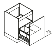
SABD Sink base unit with waste separation system
