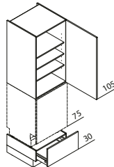
GSSA Appliance housing surround for dishwashers ↔ 60 ↓ 195/210/225 ↶ 60
