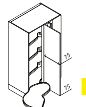
VELA Corner larder unit ↔ 110/115/125 ↓ 135/150 ↙ 60
