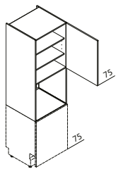
GGSB Appliance housing surround for dishwasher / oven ↔ 60 ↓ 195/210/225 ↶ 60
