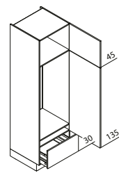
GKA Appliance unit for refrigerator / recess 122.5 cm ↔ 60 ↓ 195/210/225 ↙ 60
