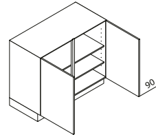
UDD Base unit ↳ 80/90/100/120 ↓ 90 ↙ 60/50/39
