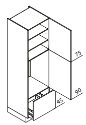
GKA Appliance unit for refrigerator / recess 88 cm ↔ 60 ↓ 195/210/225 ↙ 60
