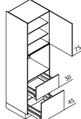
GBZ Appliance housing for oven / microwave ↔ 60 ↓ 195/210/225 ↶ 60
