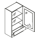
HASKV Top-mounted unit with glass door (depending on range) ↳ 45/50/60 ↓ 115 ↶ 35
