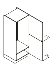
GK Appliance unit for refrigerator / recess 122.5 cm ↔ 60 ↓ 135/150 ↙ 60
