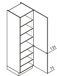
V Larder unit ↔ 30/40/45/50/60 ↓ 195/210/225 ↙ 60/50/35
