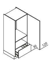
GKA Appliance unit for refrigerator / recess 88 cm ↔ 60 ↓ 135/150 ↙ 60
