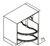
UEAD Corner base unit
