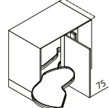
UELAD Corner base unit "LE MANS"
