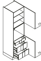
GBI Appliance housing for oven / microwave ↔ 60 ↓ 195/210/225 ↶ 60
