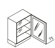
UDDDN Base unit with glass door DN ↳ 40/45/50/60 ↓ 75/90 ↙ 39
