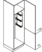
VB Broom cupboard ↔ 30/40/45/50/60 ↓ 195/210/225 ↙ 60/50
