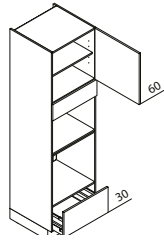
GBBA Appliance housing for oven / microwave ↔ 60 ↓ 195/210/225 ↶ 60
