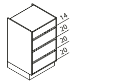
URI Base unit shelf with drawers ↳ 60/90 ↓ 90 ↙ 60/39
