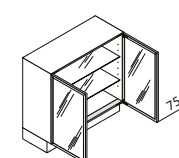
UDDDR Base unit with glass door DR ↳ 80/90/100/120 ↓ 75/90 ↙ 39
