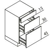
UAK Pull-out unit ↳ 30/40/45/50/60/80/90/100/120 ↓ 90 ↙ 60/50/39
