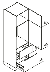
GKZ Appliance unit for refrigerator / recess 88 cm ↔ 60 ↓ 195/210/225 ↙ 60
