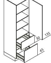
VZ Larder unit ↔ 30/40/45/50/60 ↓ 195/210/225 ↙ 60/50
