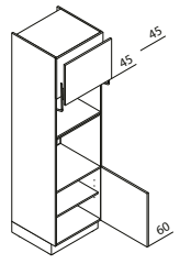
GBL Appliance housing with lift-up door for oven / microwave ↔ 60 ↓ 195/210/225 ↶ 60
