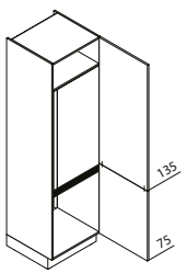
GK Appliance unit for refrigerator / recess 178 cm ↔ 60 ↓ 195/210/225 ↙ 60
