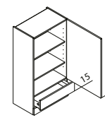
HASK Top-mounted unit ↳ 45/50/60 ↓ 115/ ↶ 35
