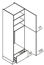
GKA Appliance unit for refrigerator / recess 102.5 cm ↔ 60 ↓ 195/210/225 ↙ 60
