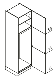
GK Appliance unit for refrigerator / recess 144 cm ↔ 60 ↓ 195/210/225 ↙ 60
