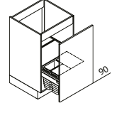
SABHD Sink base unit with waste separation system ↳ 45/50/60 ↓ 90 ↙ 60
