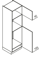
GKB Appliance housing for refrigerator and oven / recess 88 mm ↔ 60 ↓ 195/210/225 ↶ 60
