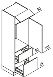
GKZ Appliance unit for refrigerator / recess 102.5 cm ↔ 60 ↓ 195/210/225 ↙ 60
