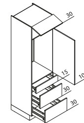
GKAK Appliance unit for refrigerator / recess 102.5 cm ↔ 60 ↓ 195/210/225 ↙ 60
