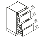
VAK Larder unit ↳ 30/40/45/50/60 ↓ 105 ↶ 60/50
