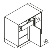
UEEA Corner base unit
