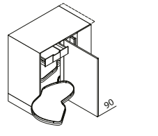
UELADI Space filler corner base unit, "LE MANS" ↳ 110/115/125 ↓ 90 ↙ 60
