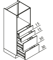
GBAP Appliance housing for oven or microwave ↔ 60 ↓ 135/150 ↙ 60
