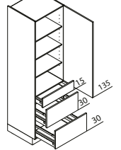
VAK Larder unit ↔ 30/40/45/50/60 ↓ 195/210/225 ↙ 60/50
