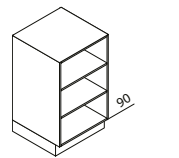
UR Open shelf base unit ↳ 15/20/25/30/35/40/45/50/55/60 ↓ 90 ↙ 60/39
