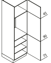
GK Appliance unit for refrigerator / recess 88 cm ↔ 60 ↓ 195/210/225 ↙ 60
