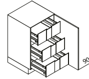
UIADD Base unit ↳ 40/45/50/60 ↓ 90 ↙ 60/50/39
