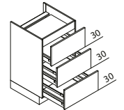
KAZ Hob base unit ↳ 60/80/90/100/120 ↓ 90 ↙ 60
